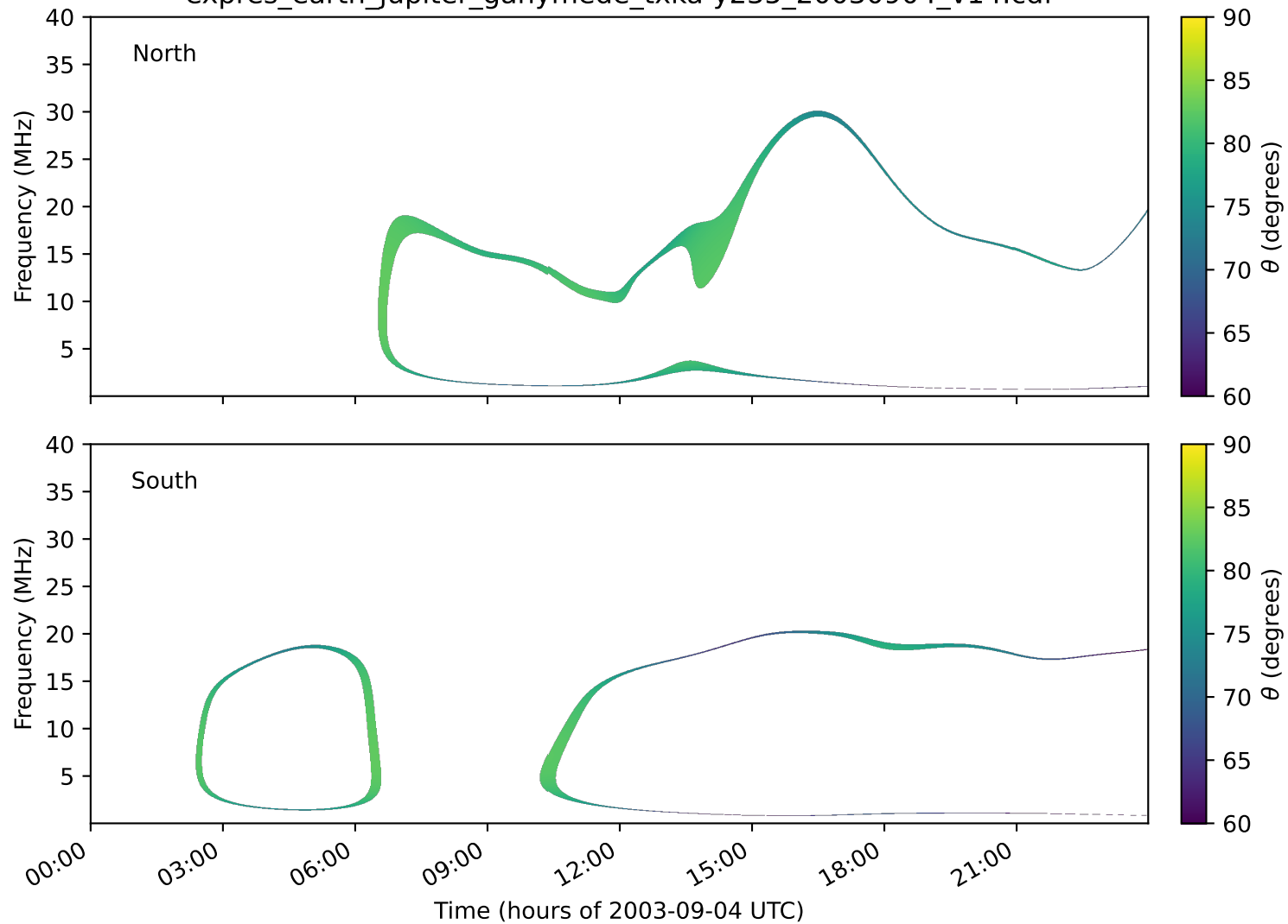
expres_earth_jupiter_ganymede_txka-y235_20030904_v14.cdf
