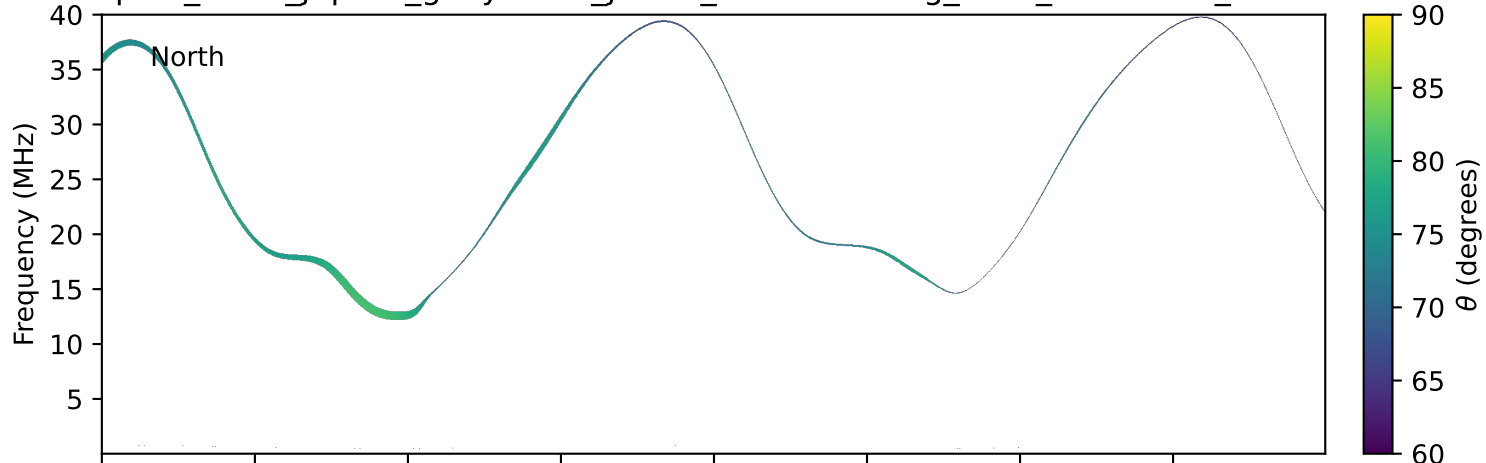
expres_earth_jupiter_ganymede_jrm33_lossc-wid1deg_3kev_20030927_v11.cdf
