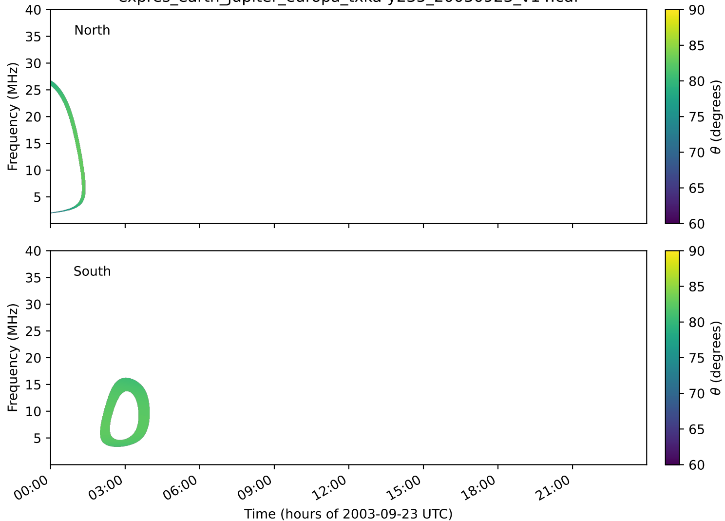
expres_earth_jupiter_europa_txka-y235_20030923_v14.cdf
