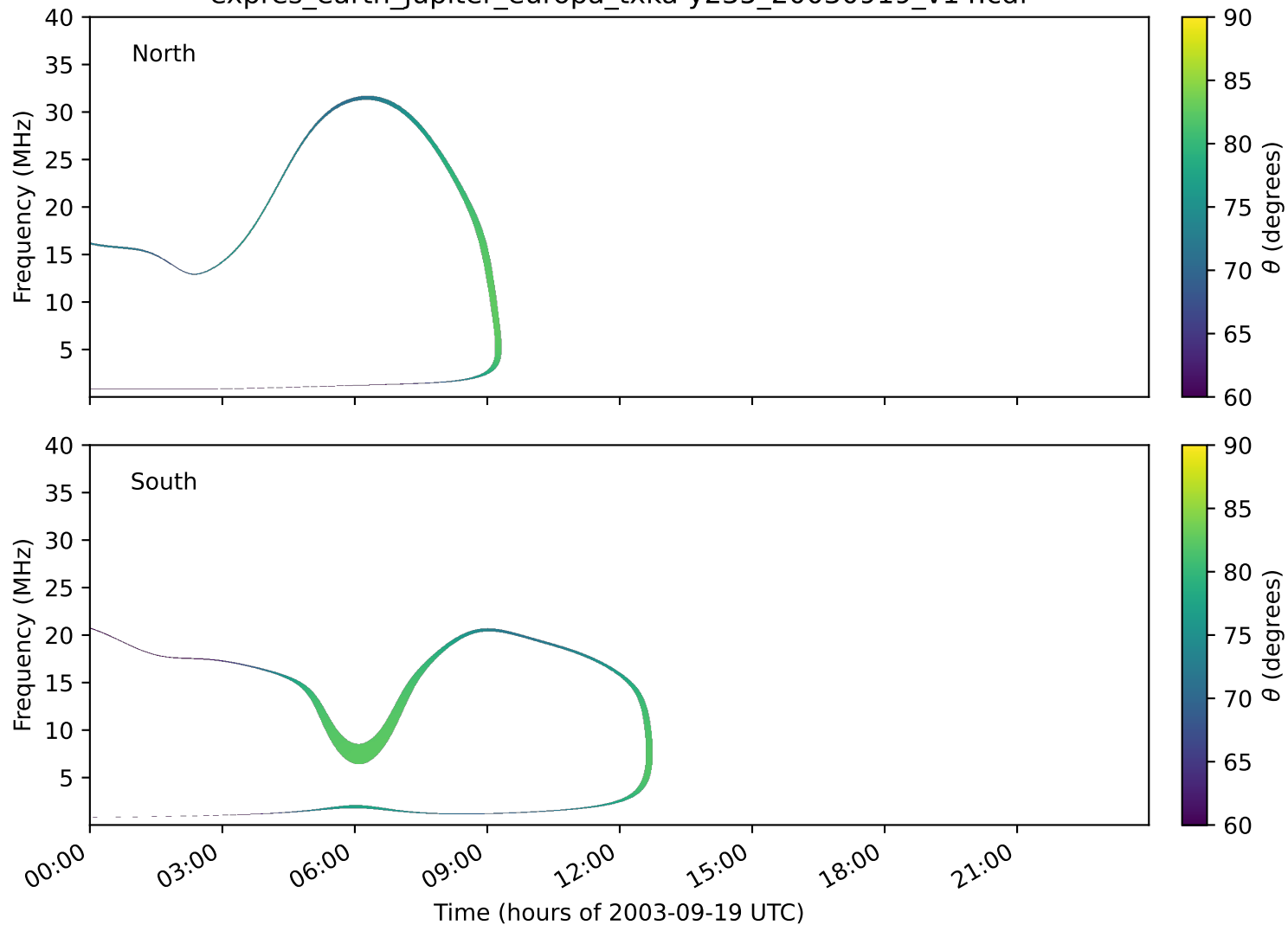
expres_earth_jupiter_europa_txka-y235_20030919_v14.cdf
