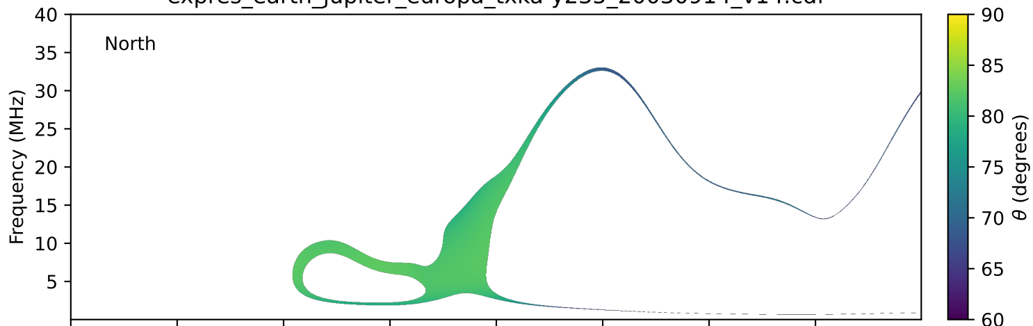
expres_earth_jupiter_europa_txka-y235_20030914_v14.cdf
