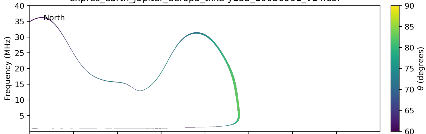
expres_earth_jupiter_europa_txka-y235_20030901_v14.cdf
