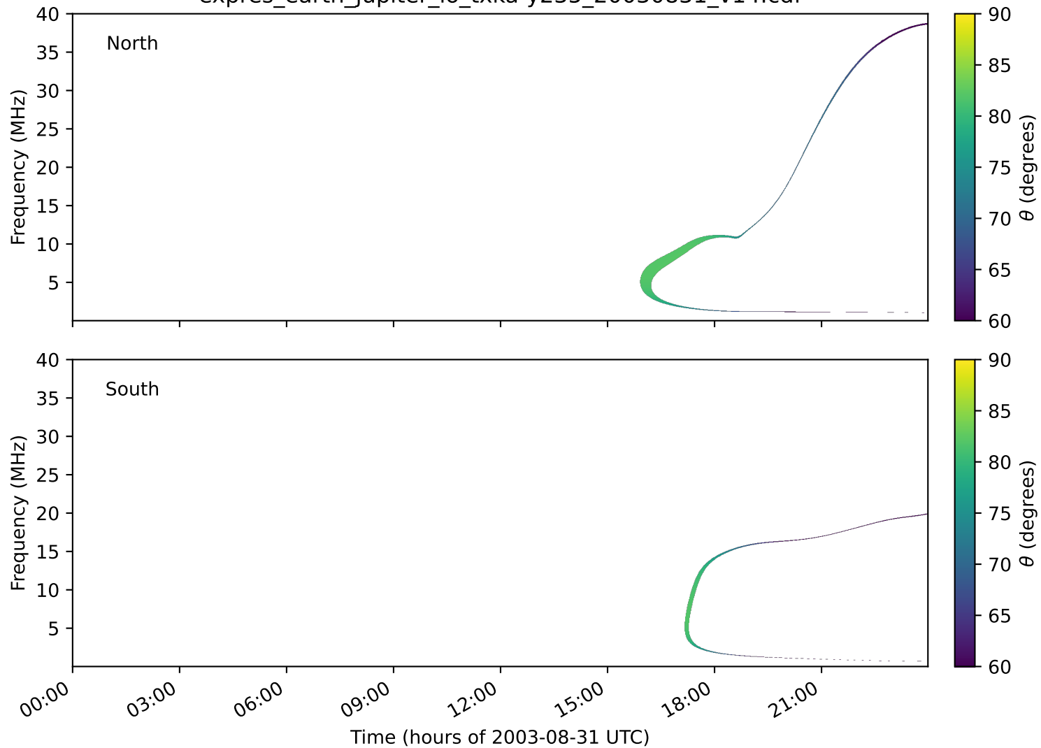
expres_earth_jupiter_io_txka-y235_20030831_v14.cdf
