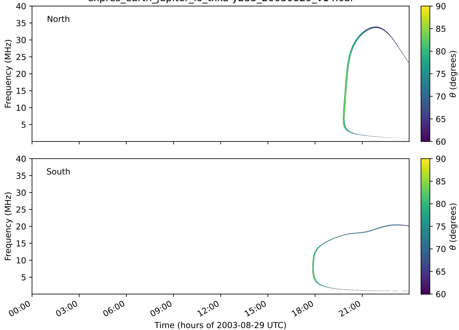
expres_earth_jupiter_io_txka-y235_20030829_v14.cdf
