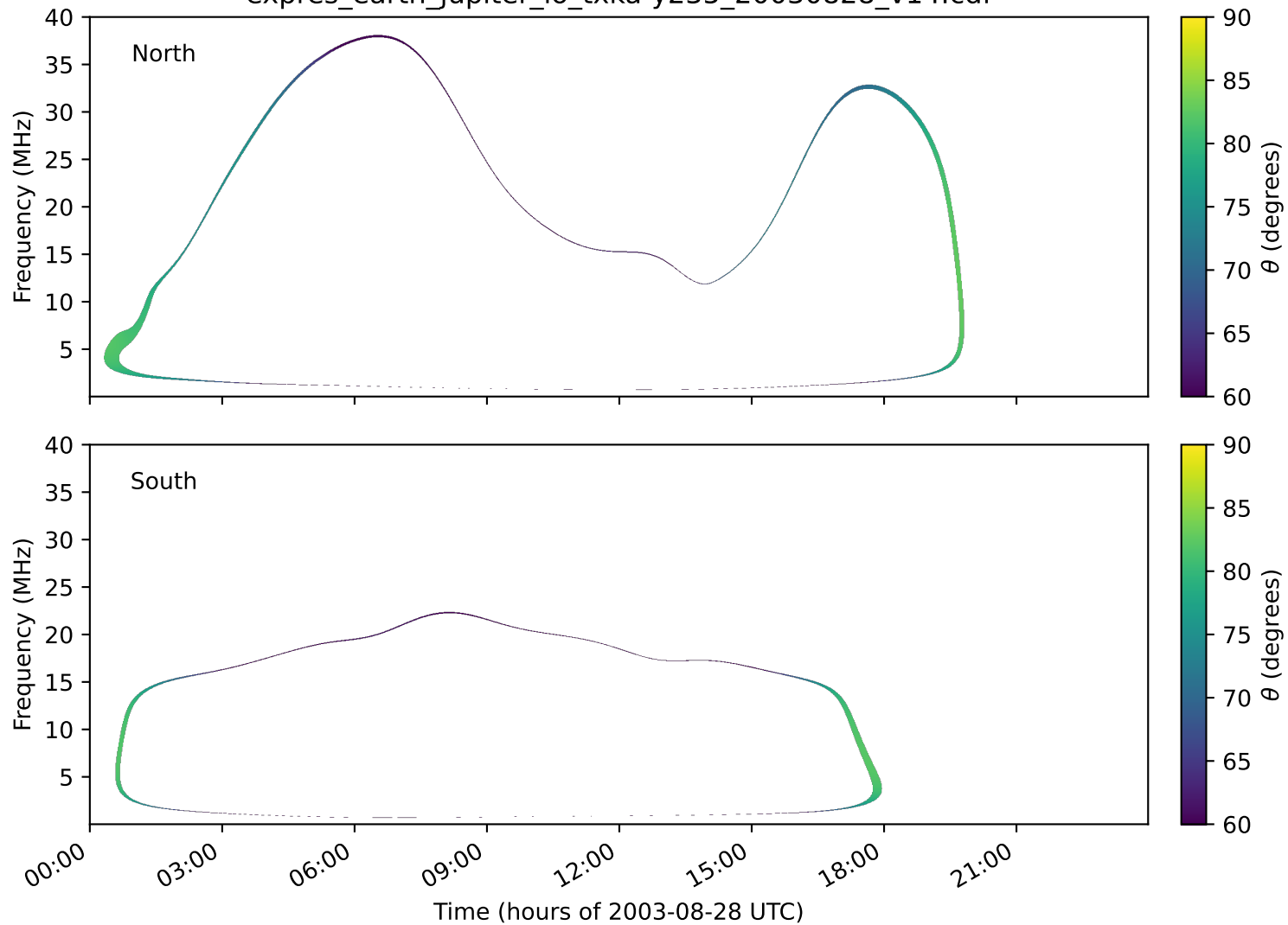
expres_earth_jupiter_io_txka-y235_20030828_v14.cdf
