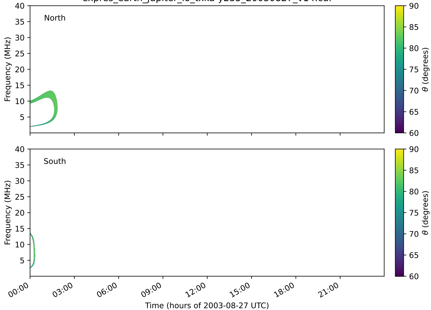
expres_earth_jupiter_io_txka-y235_20030827_v14.cdf
