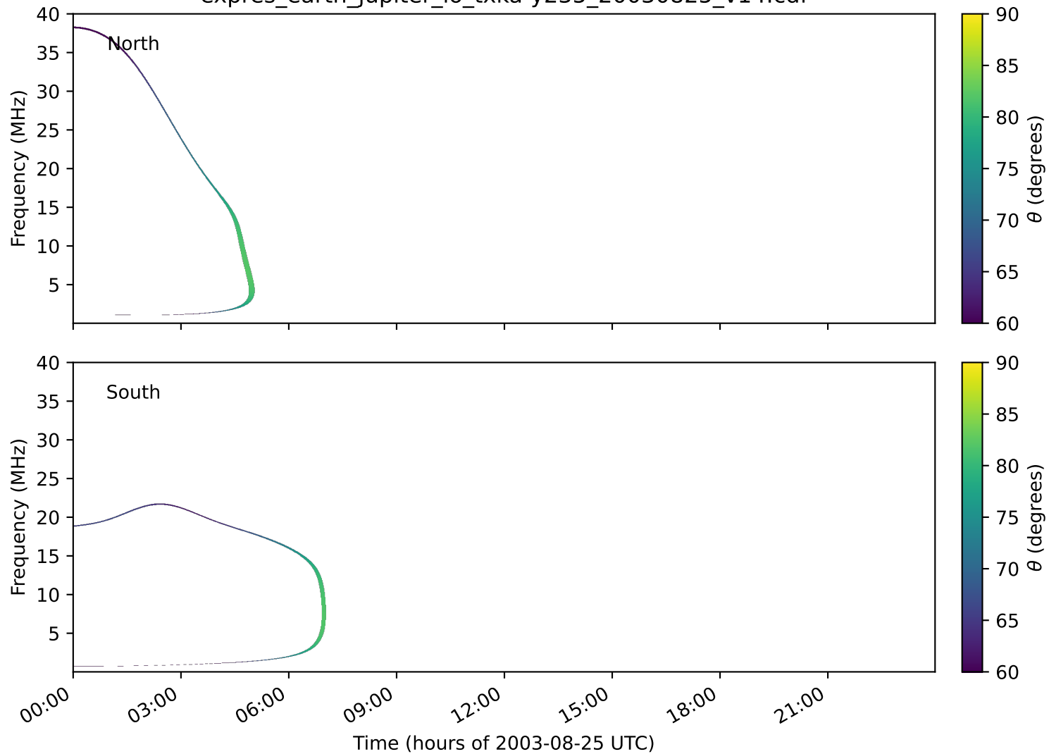
expres_earth_jupiter_io_txka-y235_20030825_v14.cdf
