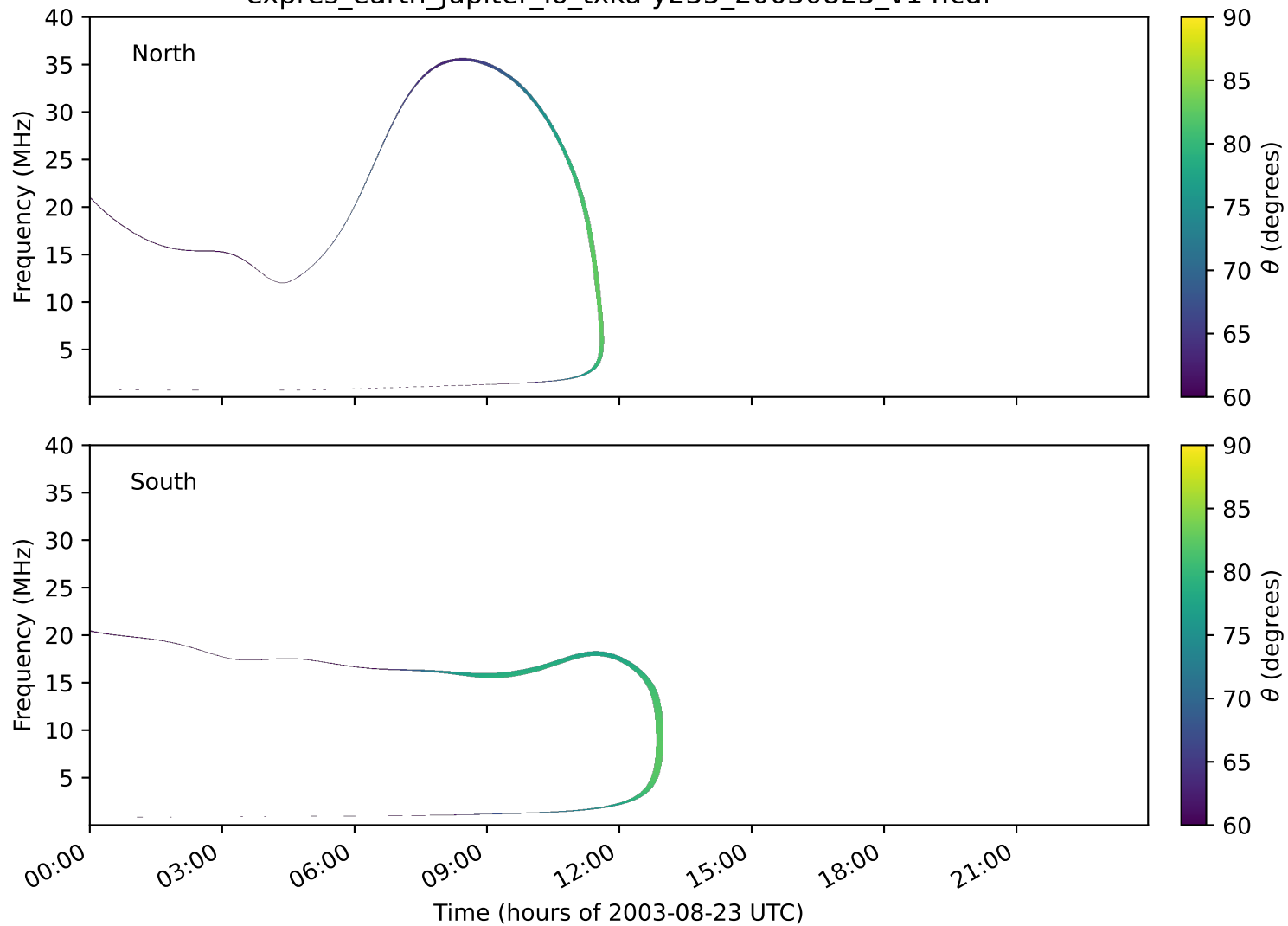
expres_earth_jupiter_io_txka-y235_20030823_v14.cdf
