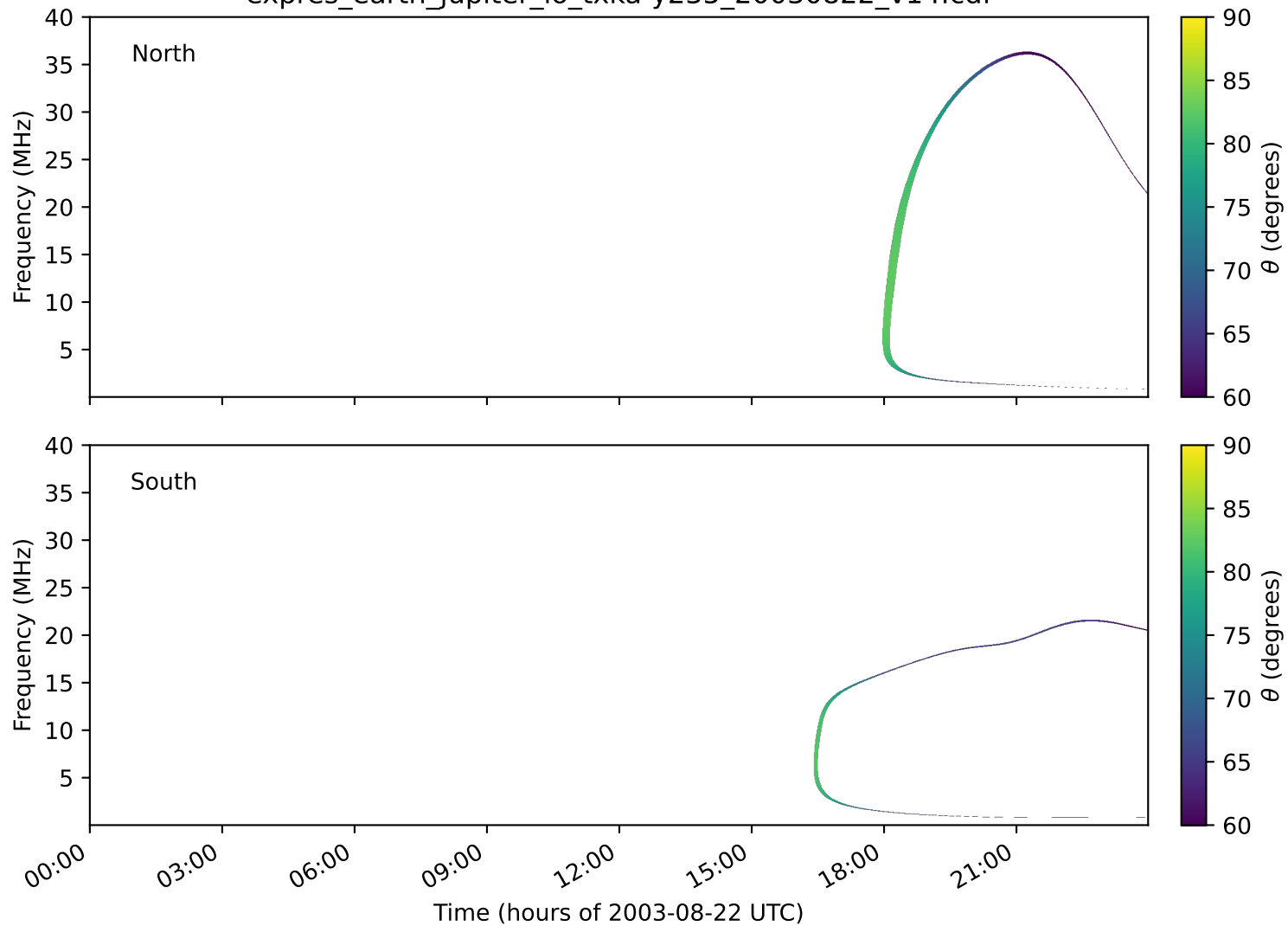
expres_earth_jupiter_io_txka-y235_20030822_v14.cdf
