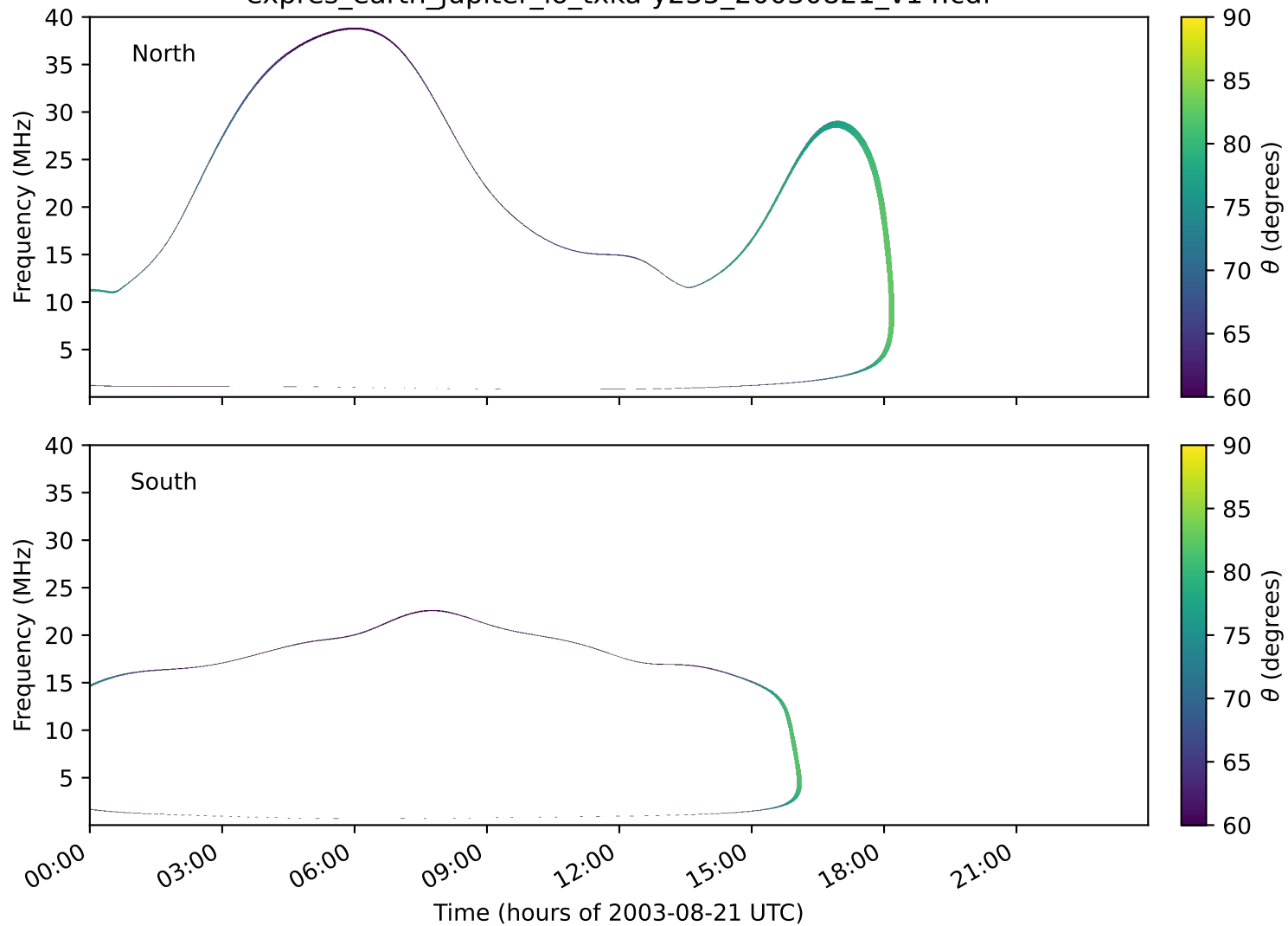
expres_earth_jupiter_io_txka-y235_20030821_v14.cdf
