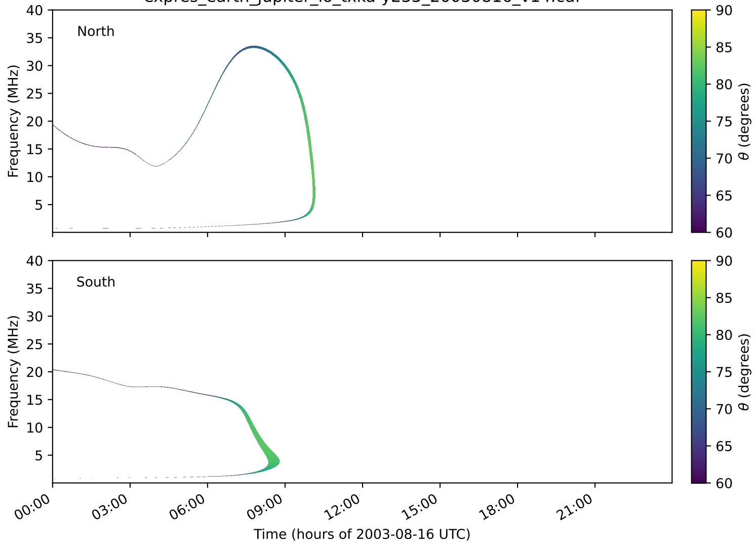
expres_earth_jupiter_io_txka-y235_20030816_v14.cdf
