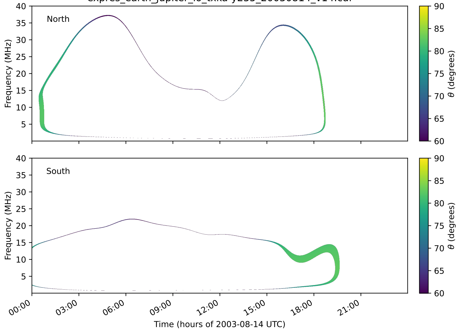
expres_earth_jupiter_io_txka-y235_20030814_v14.cdf
