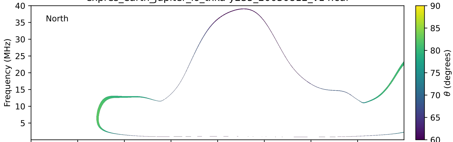
expres_earth_jupiter_io_txka-y235_20030812_v14.cdf
