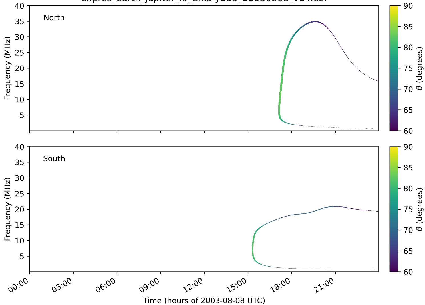
expres_earth_jupiter_io_txka-y235_20030808_v14.cdf
