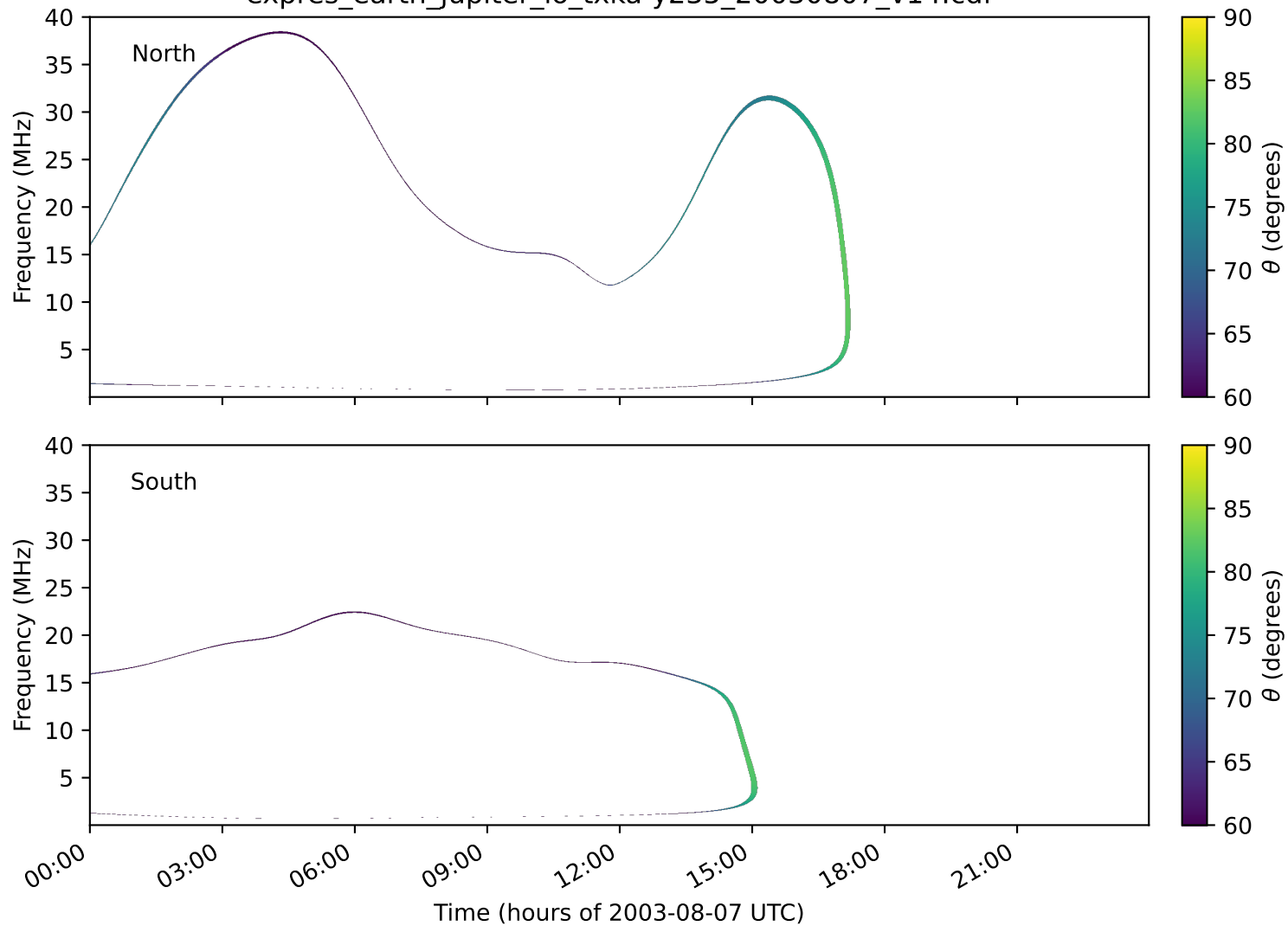
expres_earth_jupiter_io_txka-y235_20030807_v14.cdf
