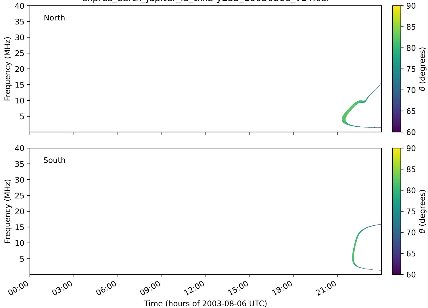
expres_earth_jupiter_io_txka-y235_20030806_v14.cdf
