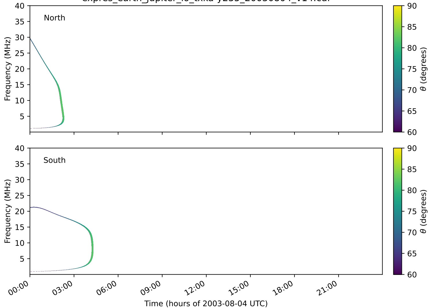
expres_earth_jupiter_io_txka-y235_20030804_v14.cdf
