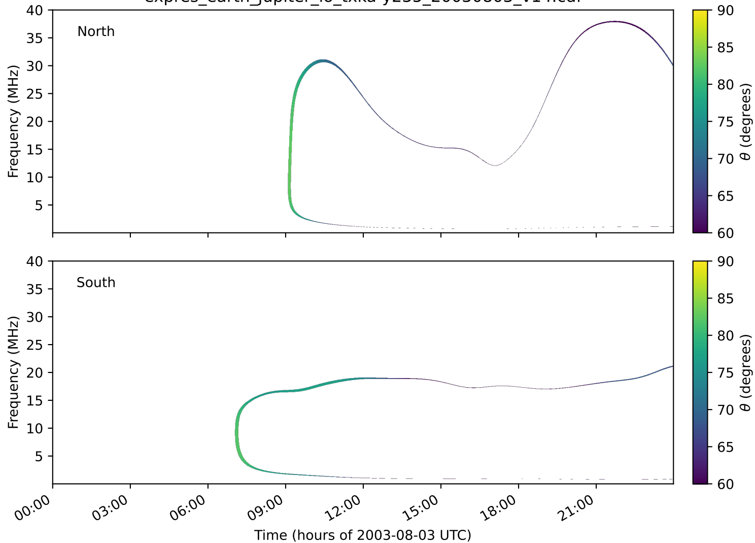
expres_earth_jupiter_io_txka-y235_20030803_v14.cdf
