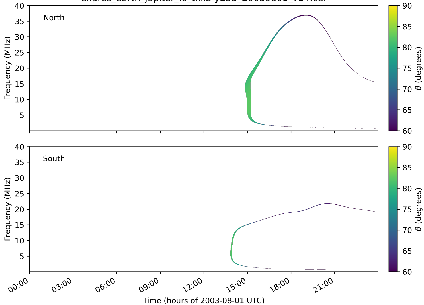
expres_earth_jupiter_io_txka-y235_20030801_v14.cdf
