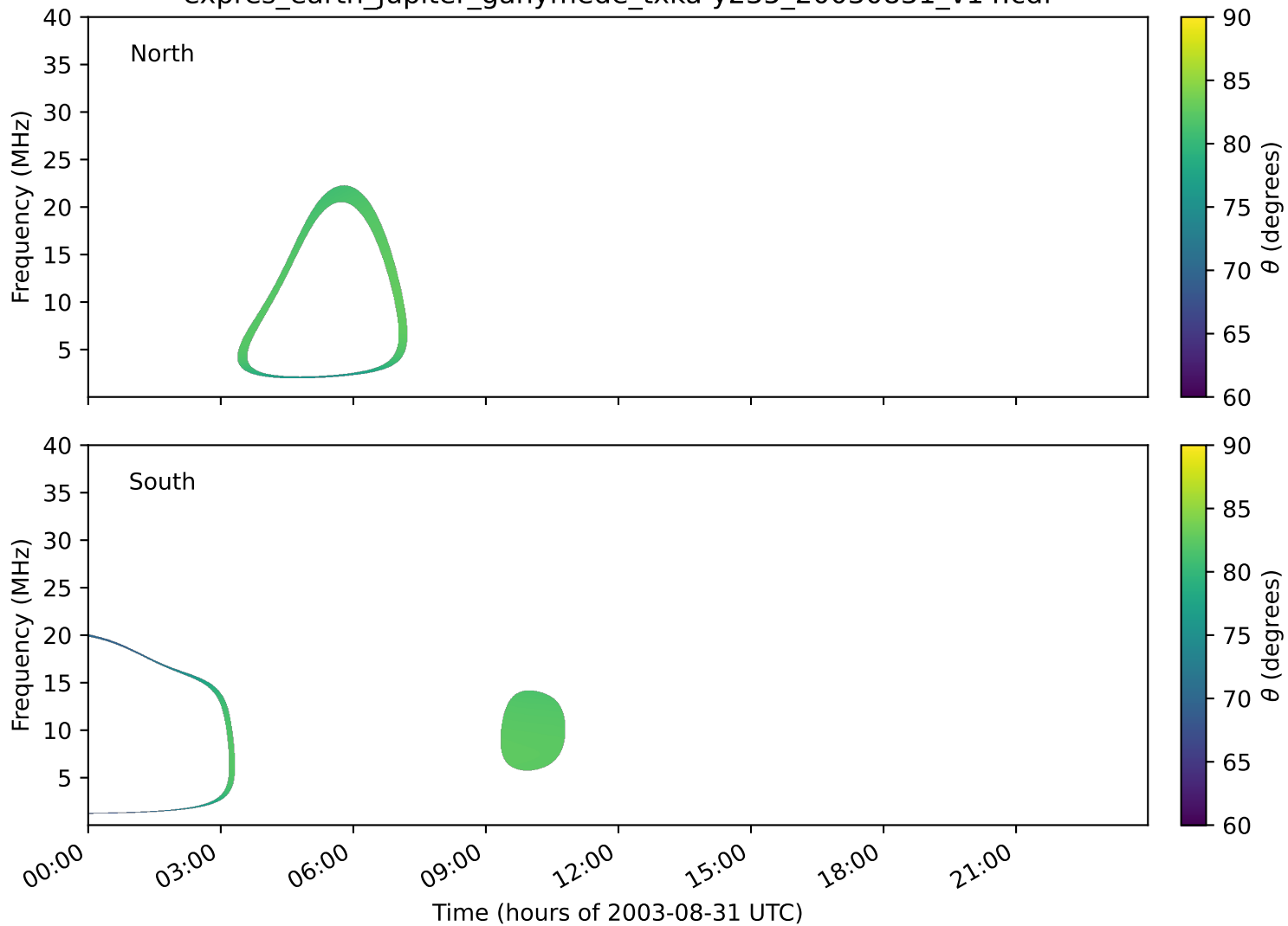
expres_earth_jupiter_ganymede_txka-y235_20030831_v14.cdf
