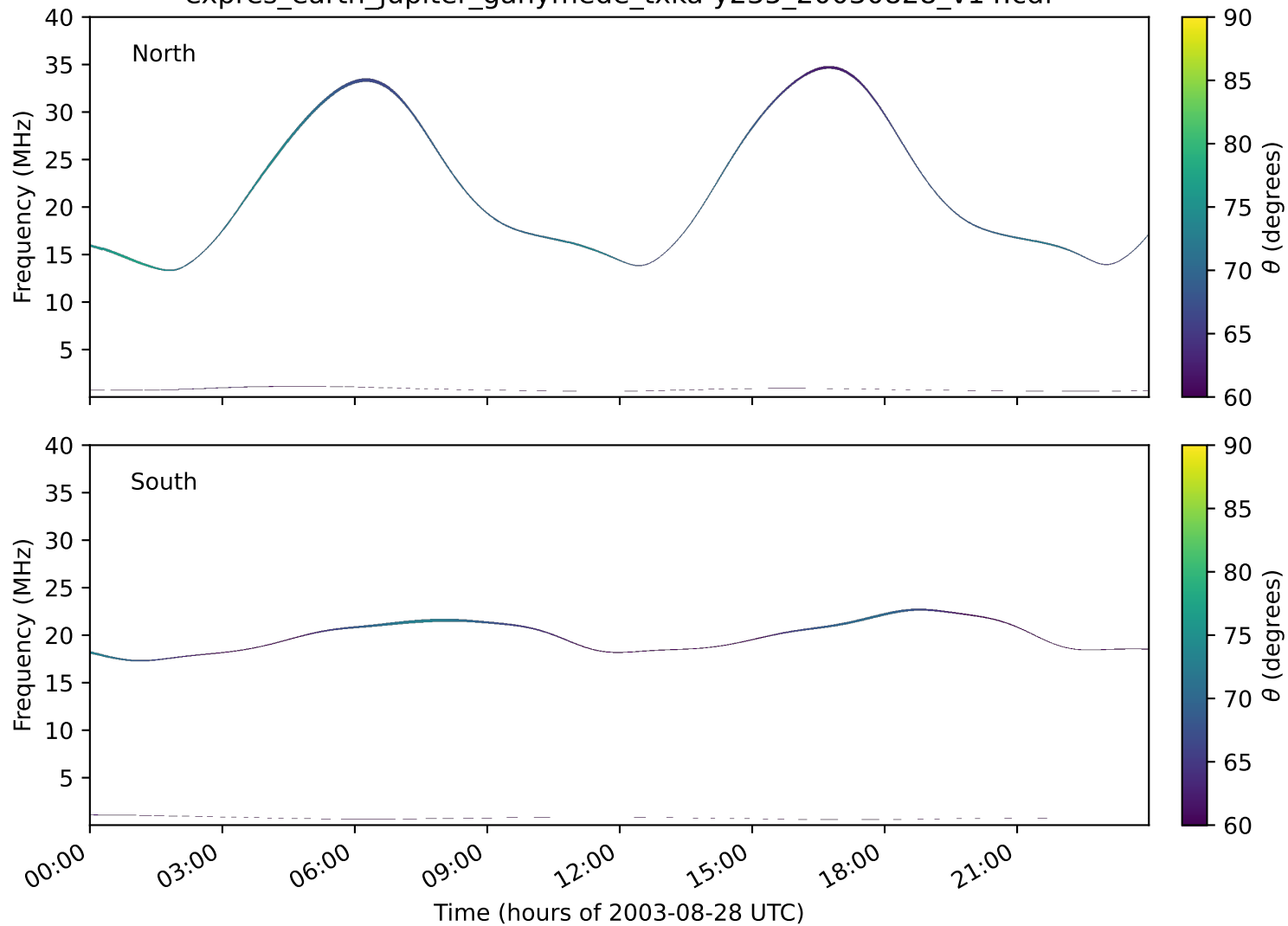
expres_earth_jupiter_ganymede_txka-y235_20030828_v14.cdf
