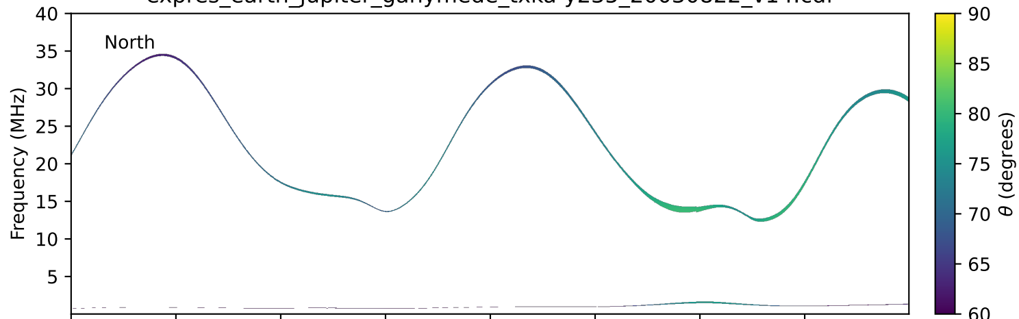
expres_earth_jupiter_ganymede_txka-y235_20030822_v14.cdf
