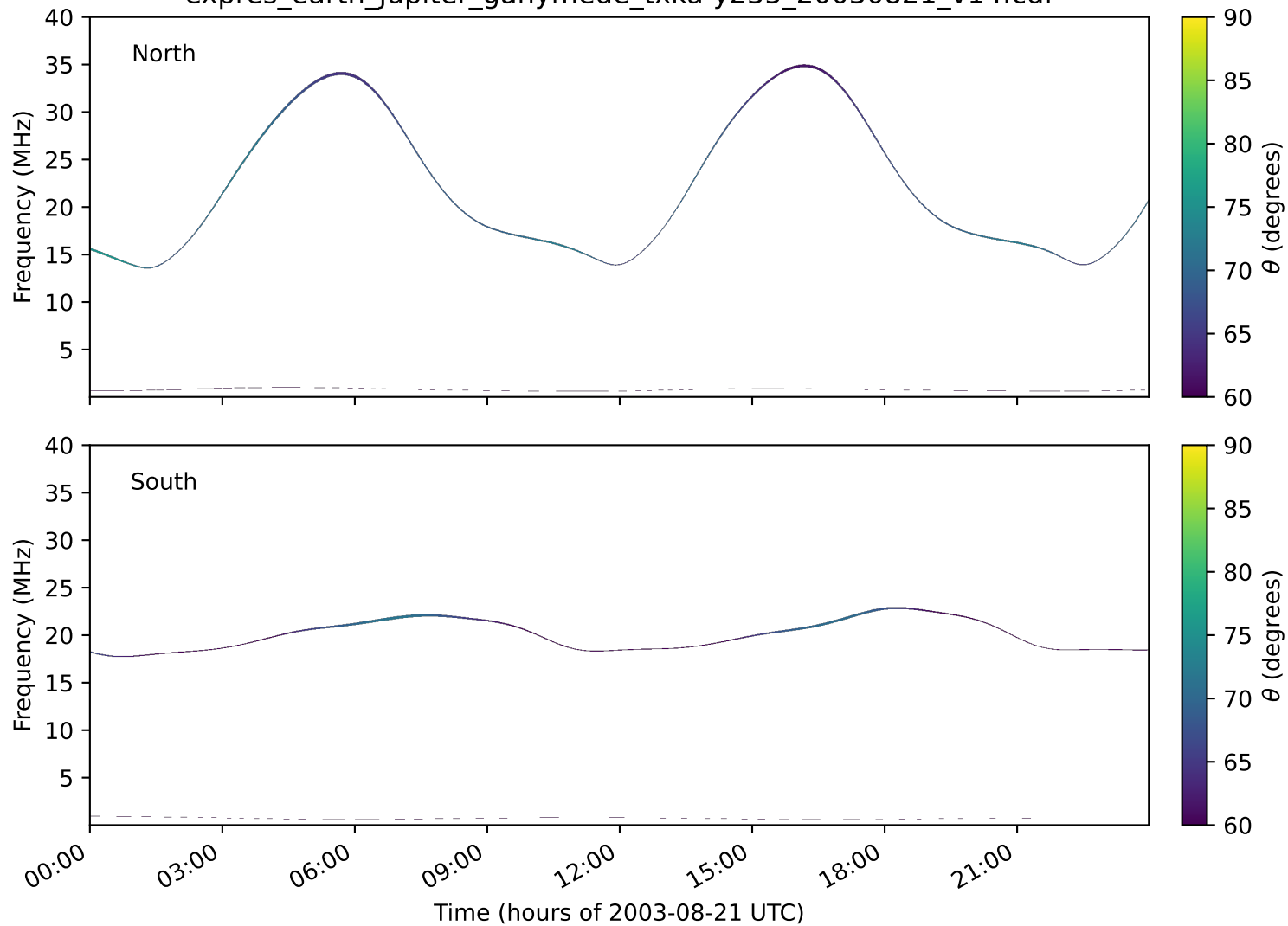
expres_earth_jupiter_ganymede_txka-y235_20030821_v14.cdf
