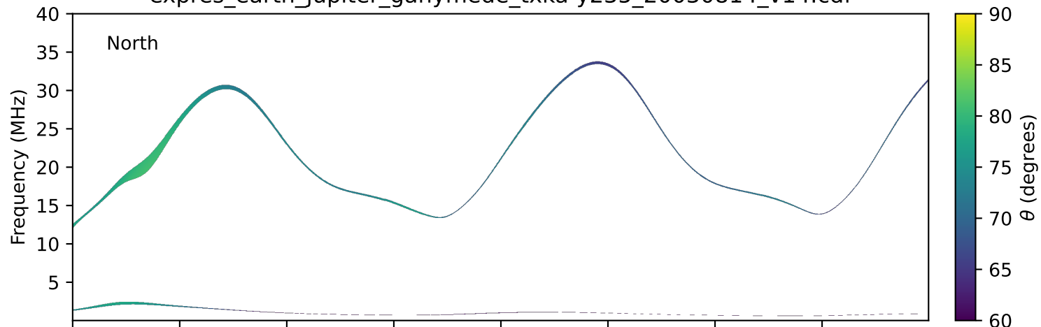
expres_earth_jupiter_ganymede_txka-y235_20030814_v14.cdf
