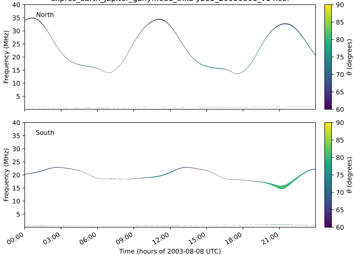
expres_earth_jupiter_ganymede_txka-y235_20030808_v14.cdf
