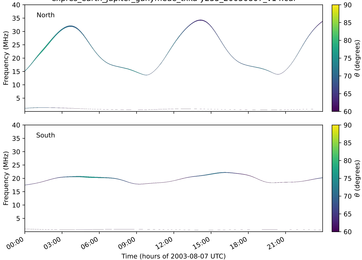
expres_earth_jupiter_ganymede_txka-y235_20030807_v14.cdf
