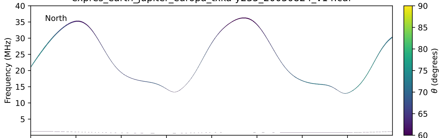
expres_earth_jupiter_europa_txka-y235_20030824_v14.cdf
