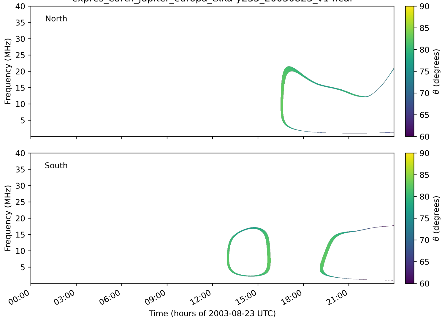
expres_earth_jupiter_europa_txka-y235_20030823_v14.cdf
