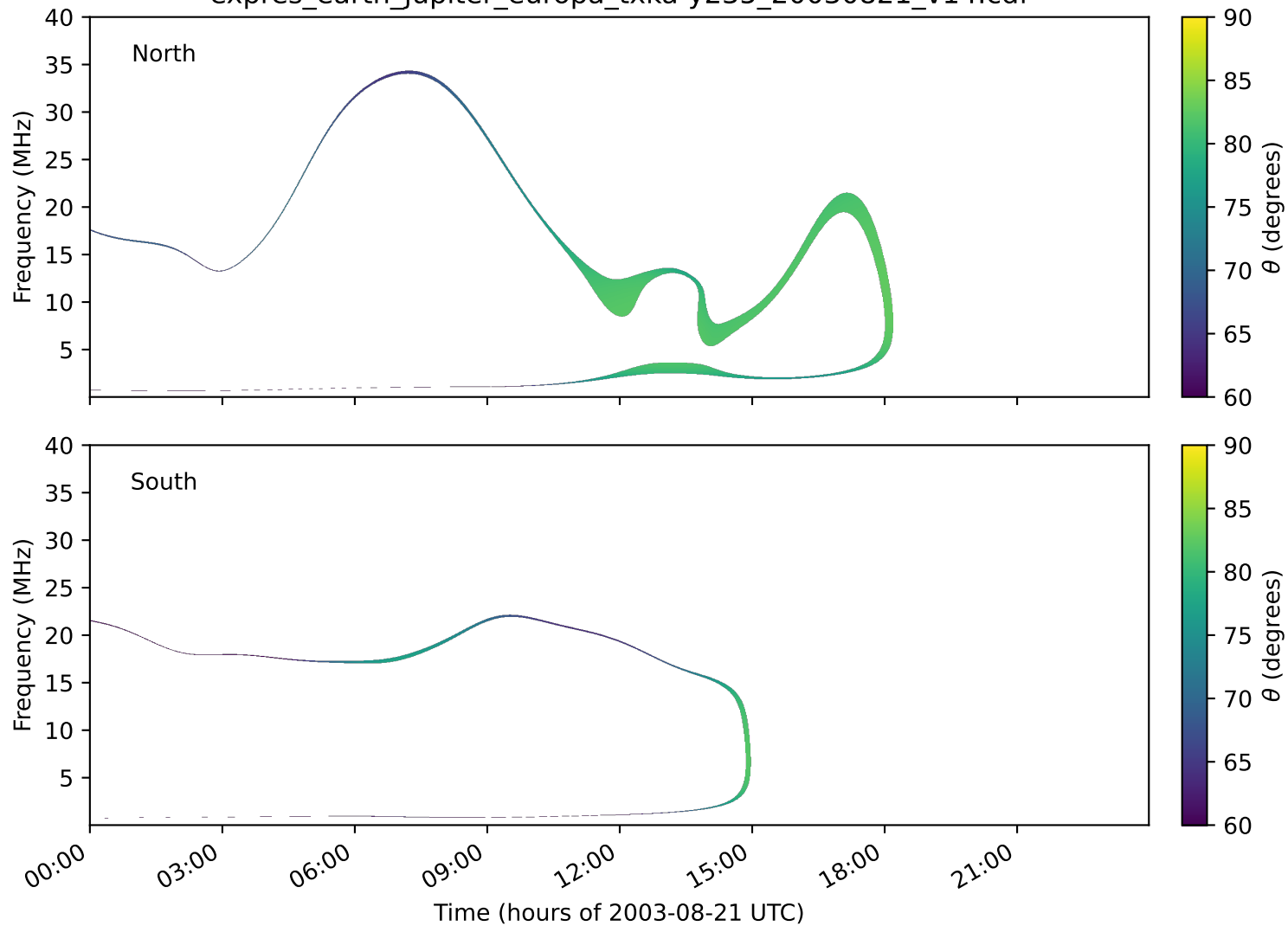
expres_earth_jupiter_europa_txka-y235_20030821_v14.cdf
