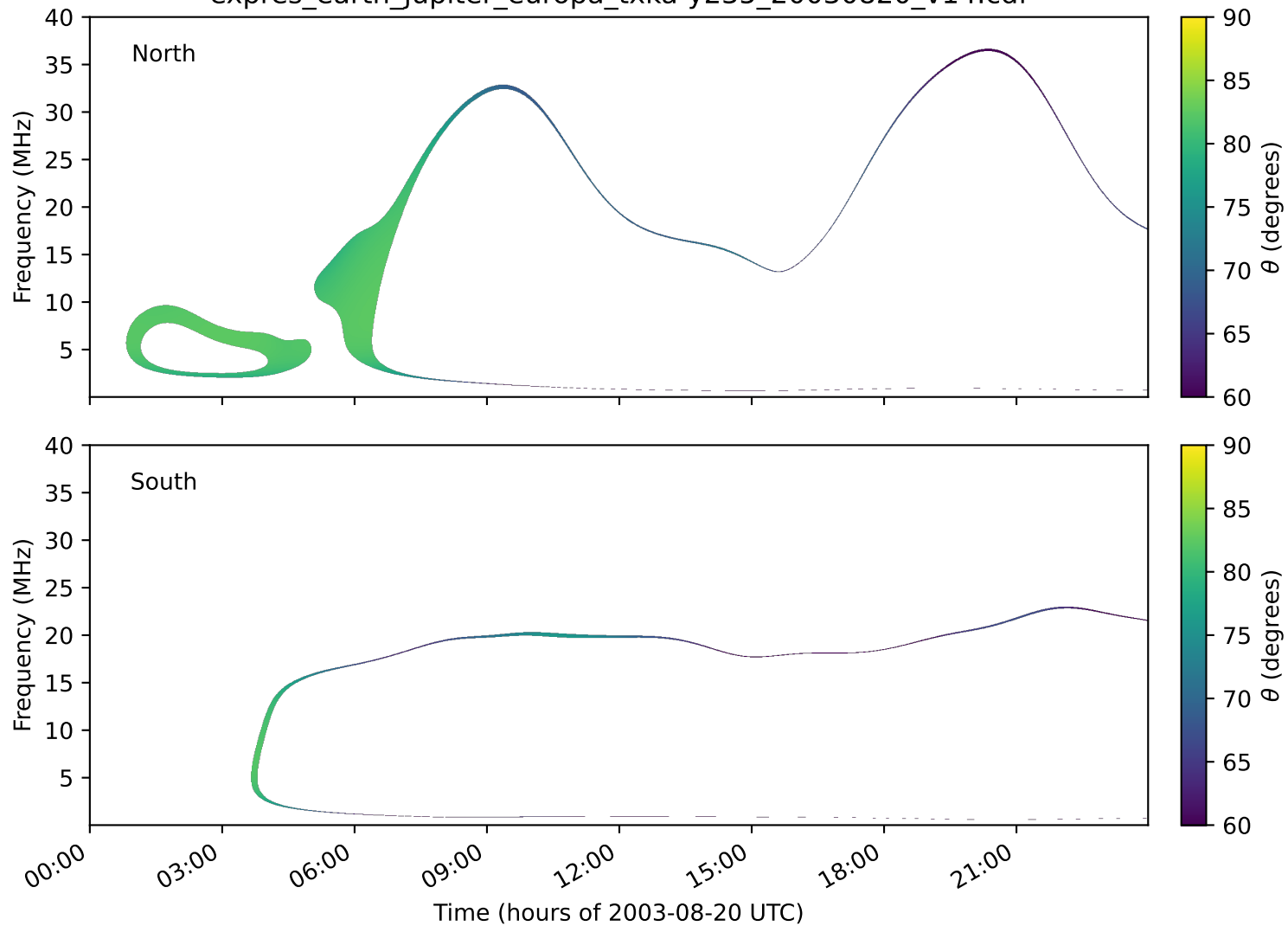
expres_earth_jupiter_europa_txka-y235_20030820_v14.cdf
