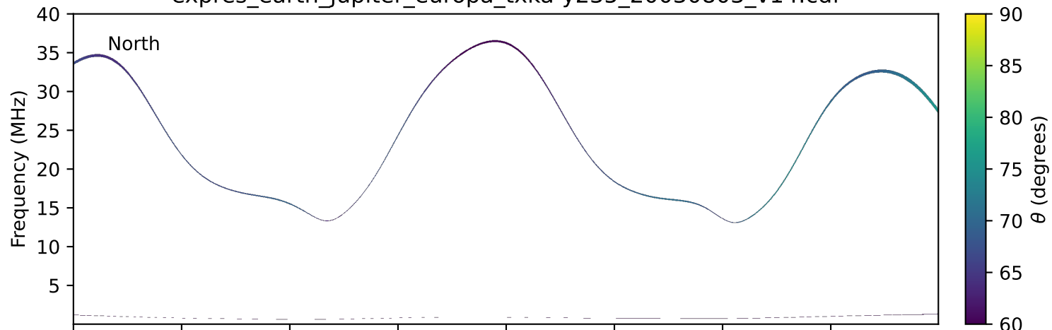
expres_earth_jupiter_europa_txka-y235_20030803_v14.cdf
