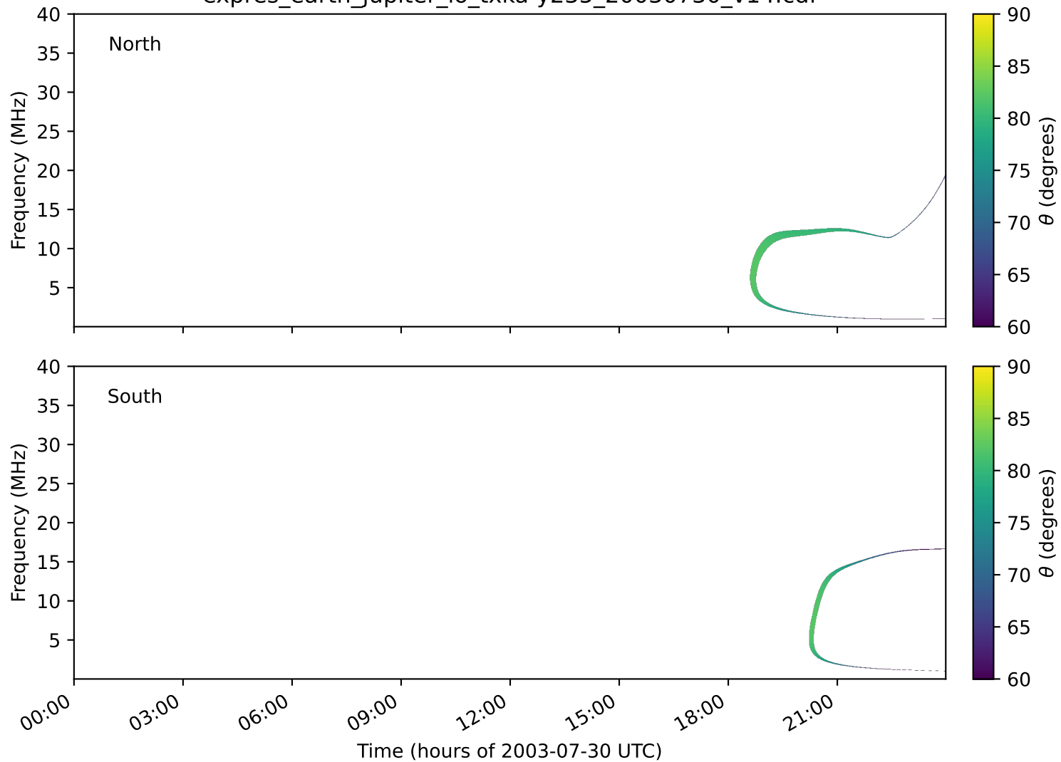
expres_earth_jupiter_io_txka-y235_20030730_v14.cdf
