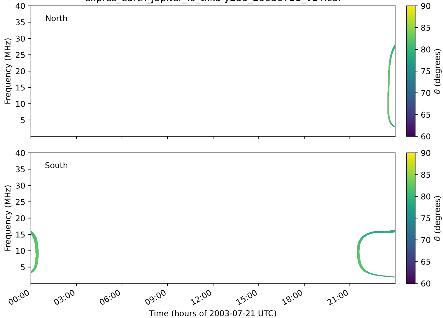
expres_earth_jupiter_io_txka-y235_20030721_v14.cdf
