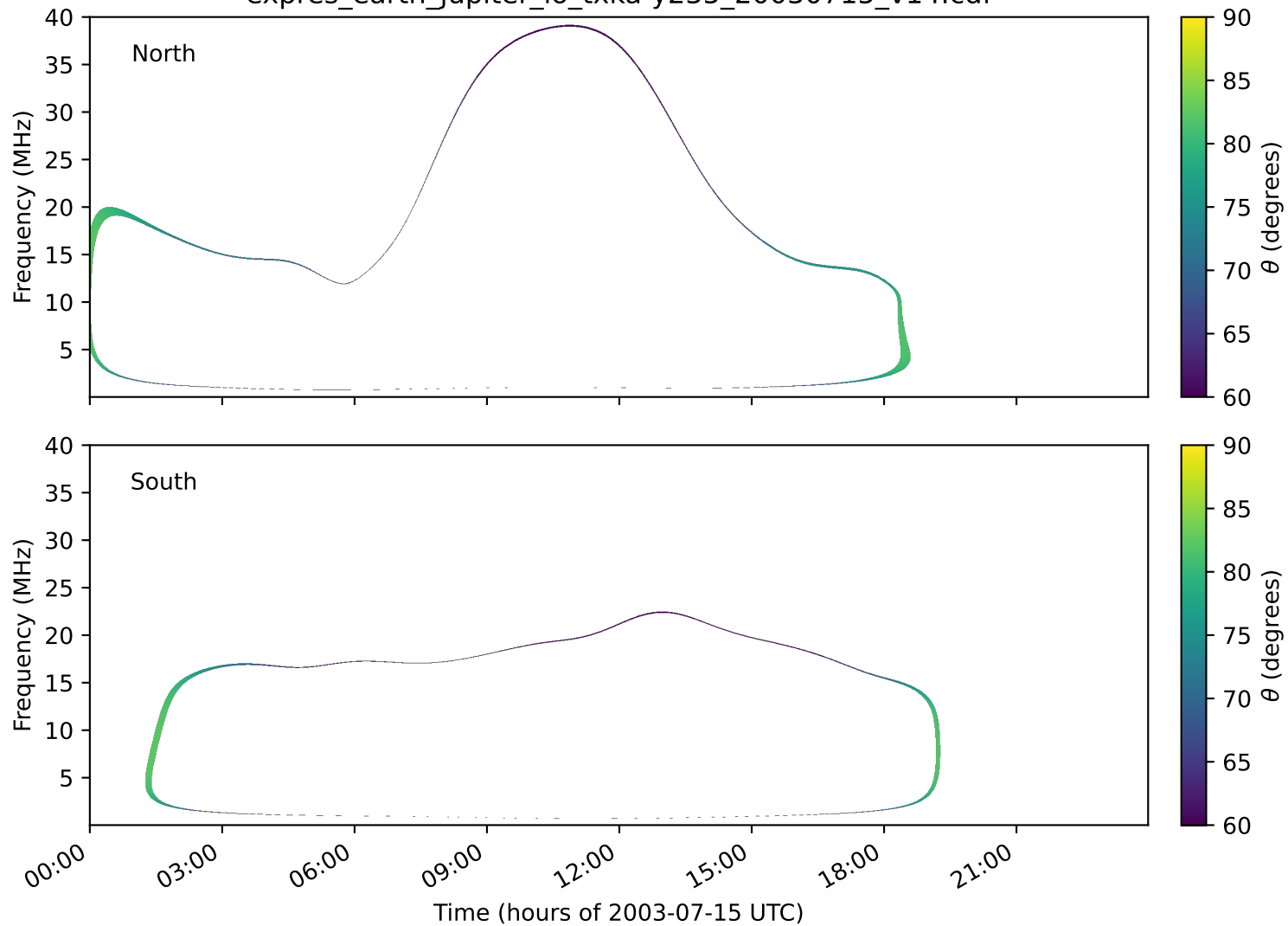
expres_earth_jupiter_io_txka-y235_20030715_v14.cdf
