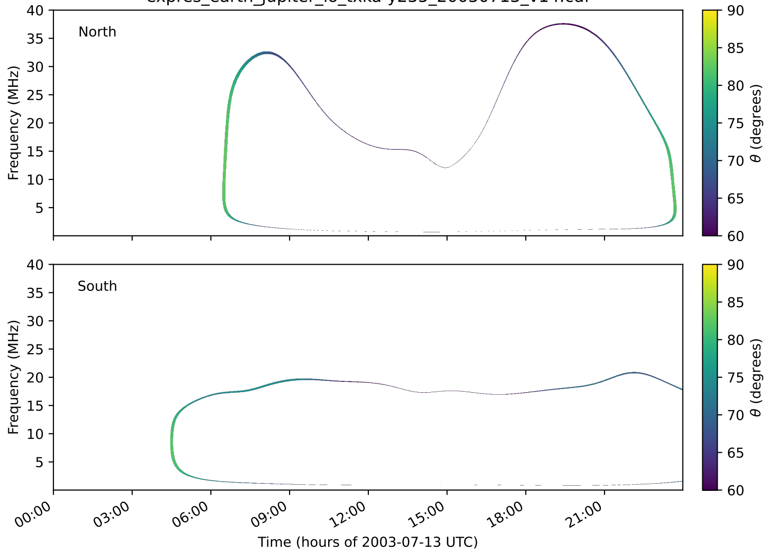
expres_earth_jupiter_io_txka-y235_20030713_v14.cdf
