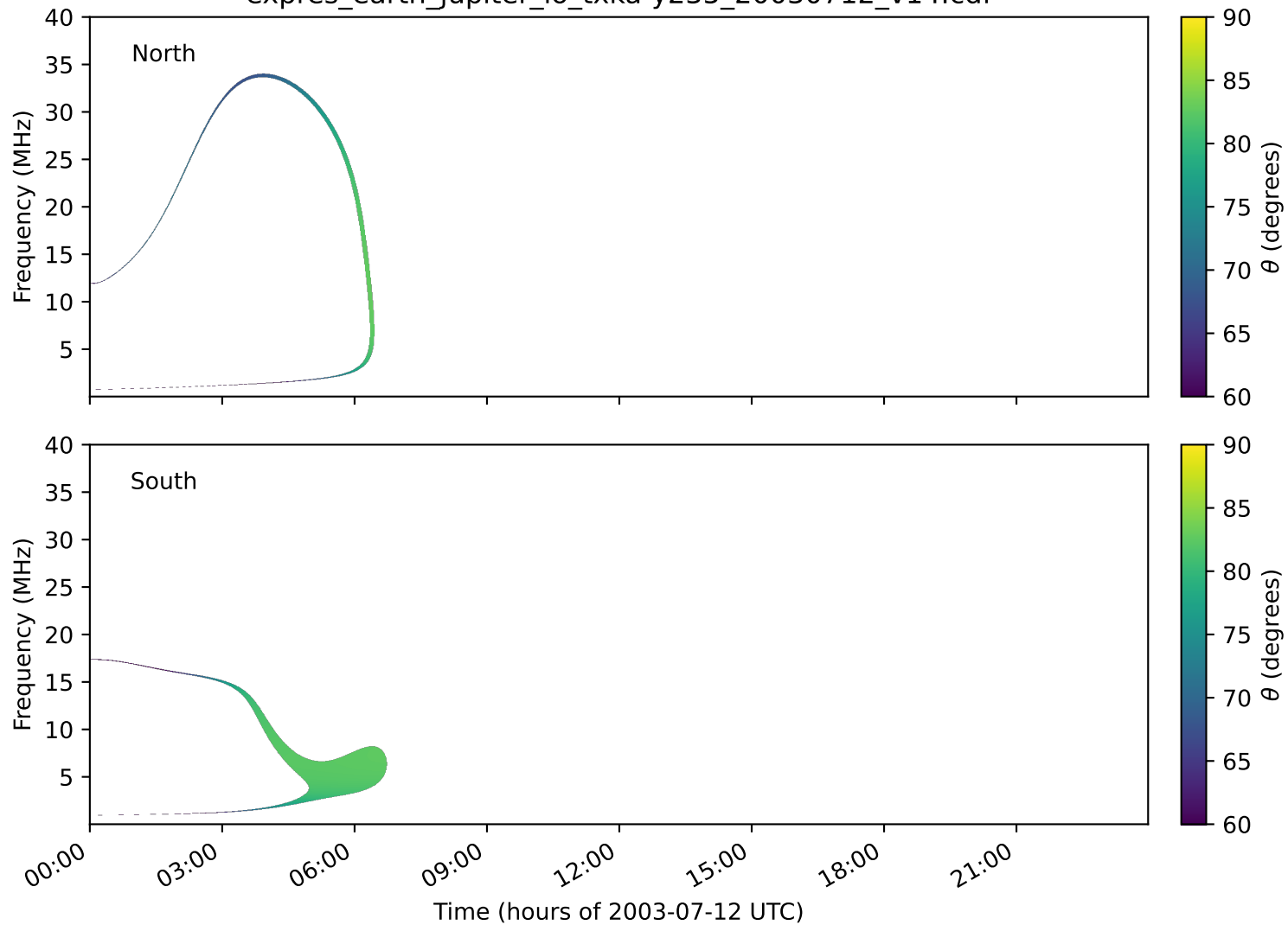
expres_earth_jupiter_io_txka-y235_20030712_v14.cdf
