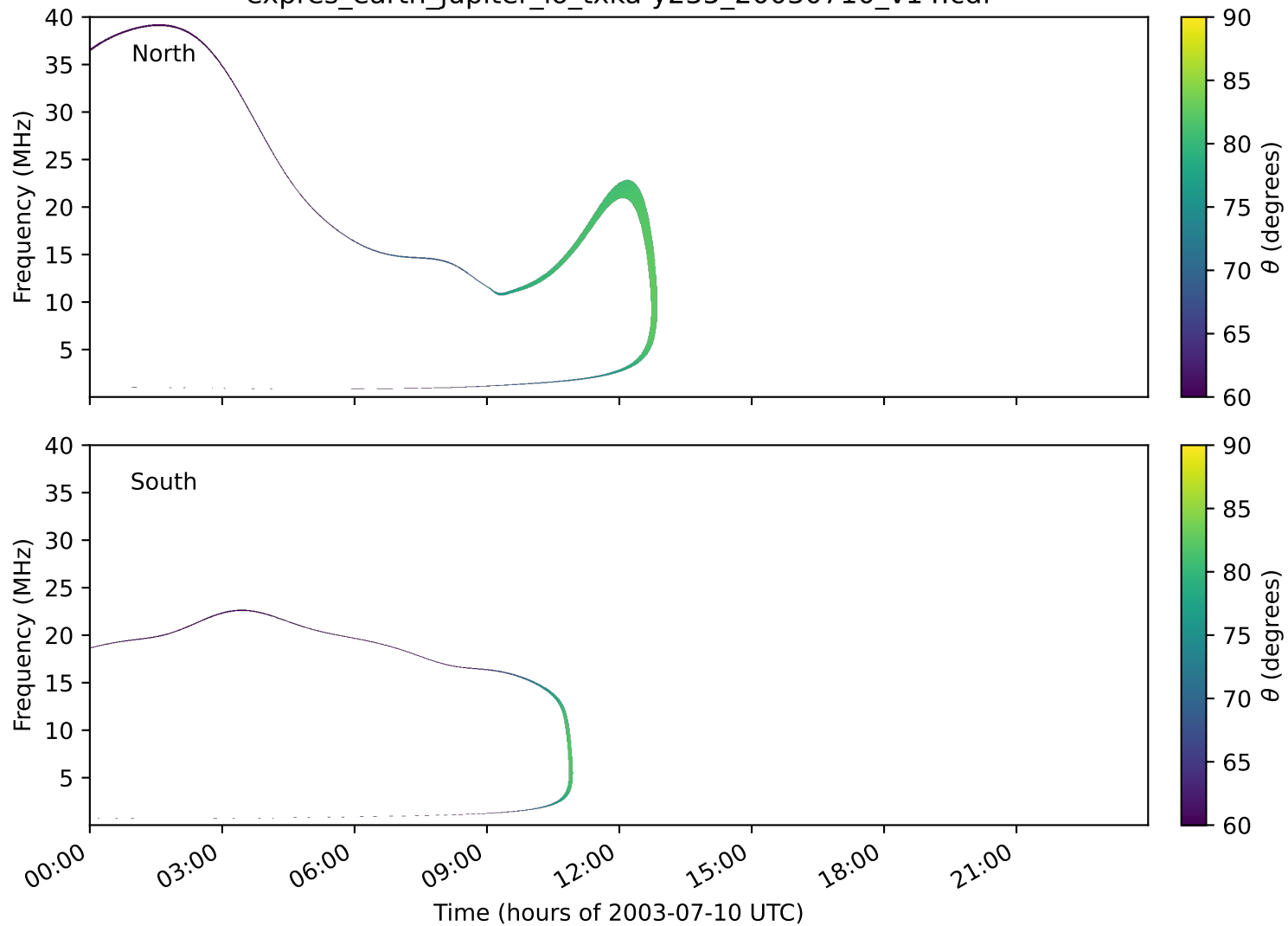
expres_earth_jupiter_io_txka-y235_20030710_v14.cdf
