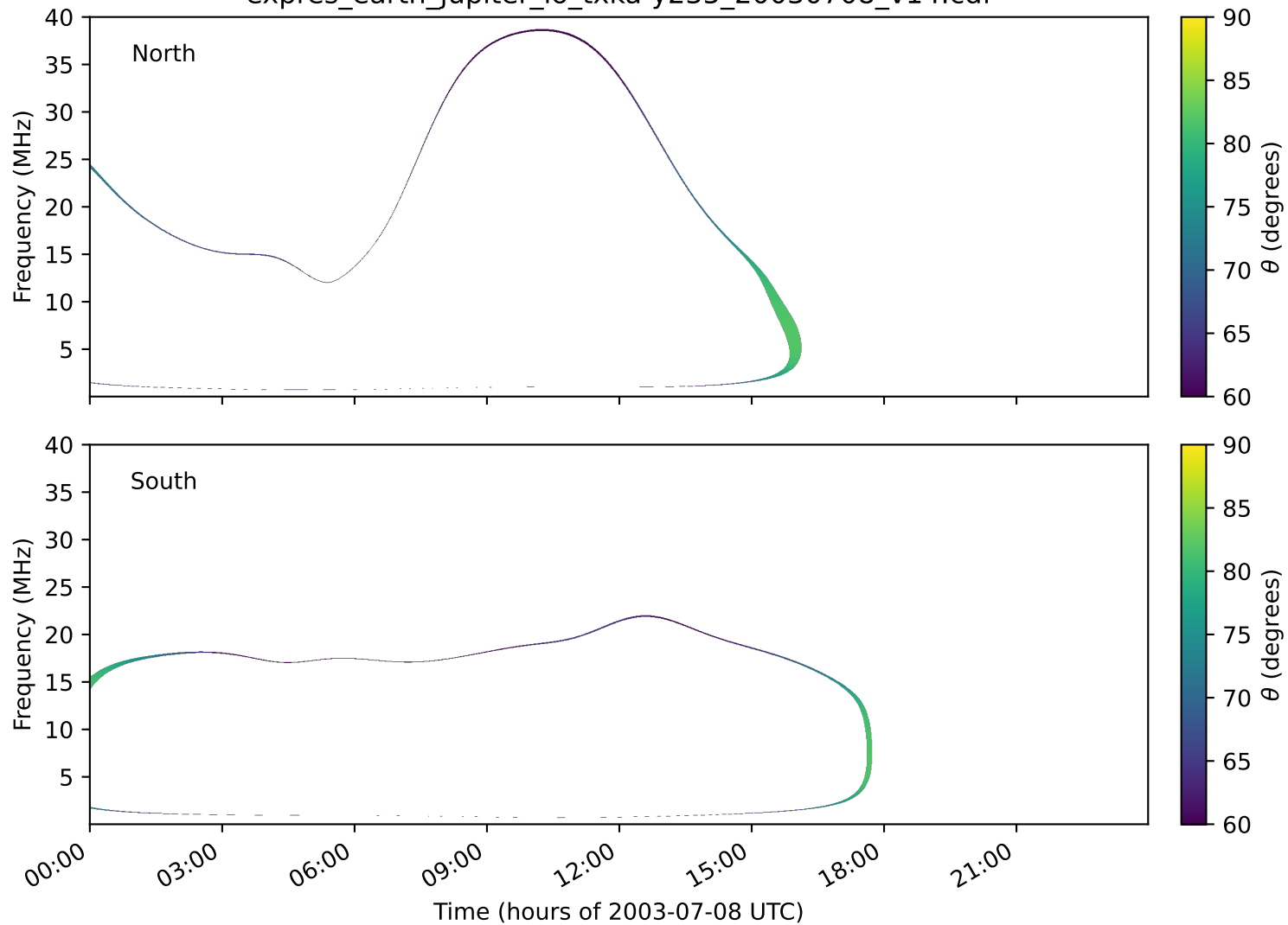
expres_earth_jupiter_io_txka-y235_20030708_v14.cdf
