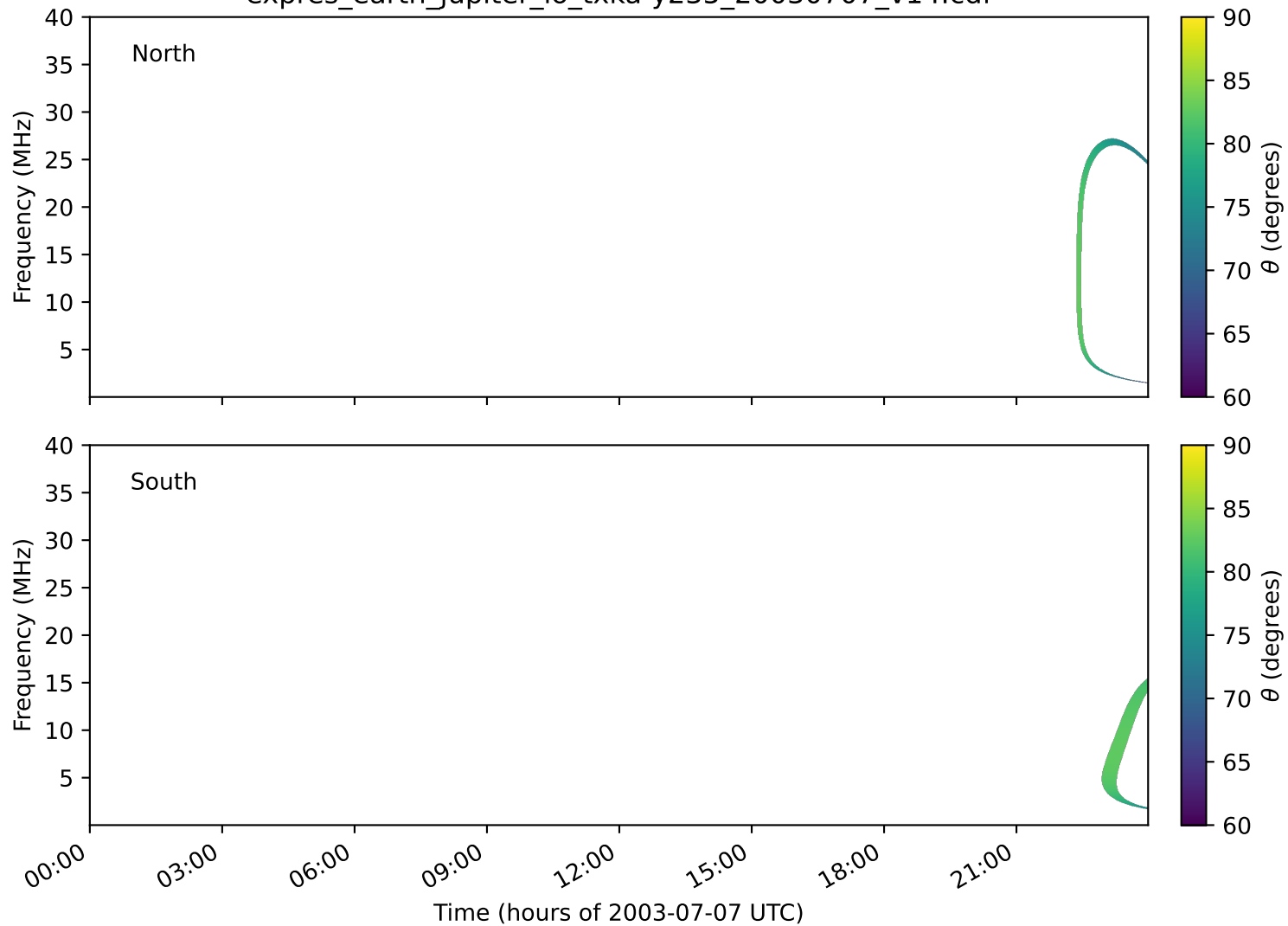
expres_earth_jupiter_io_txka-y235_20030707_v14.cdf
