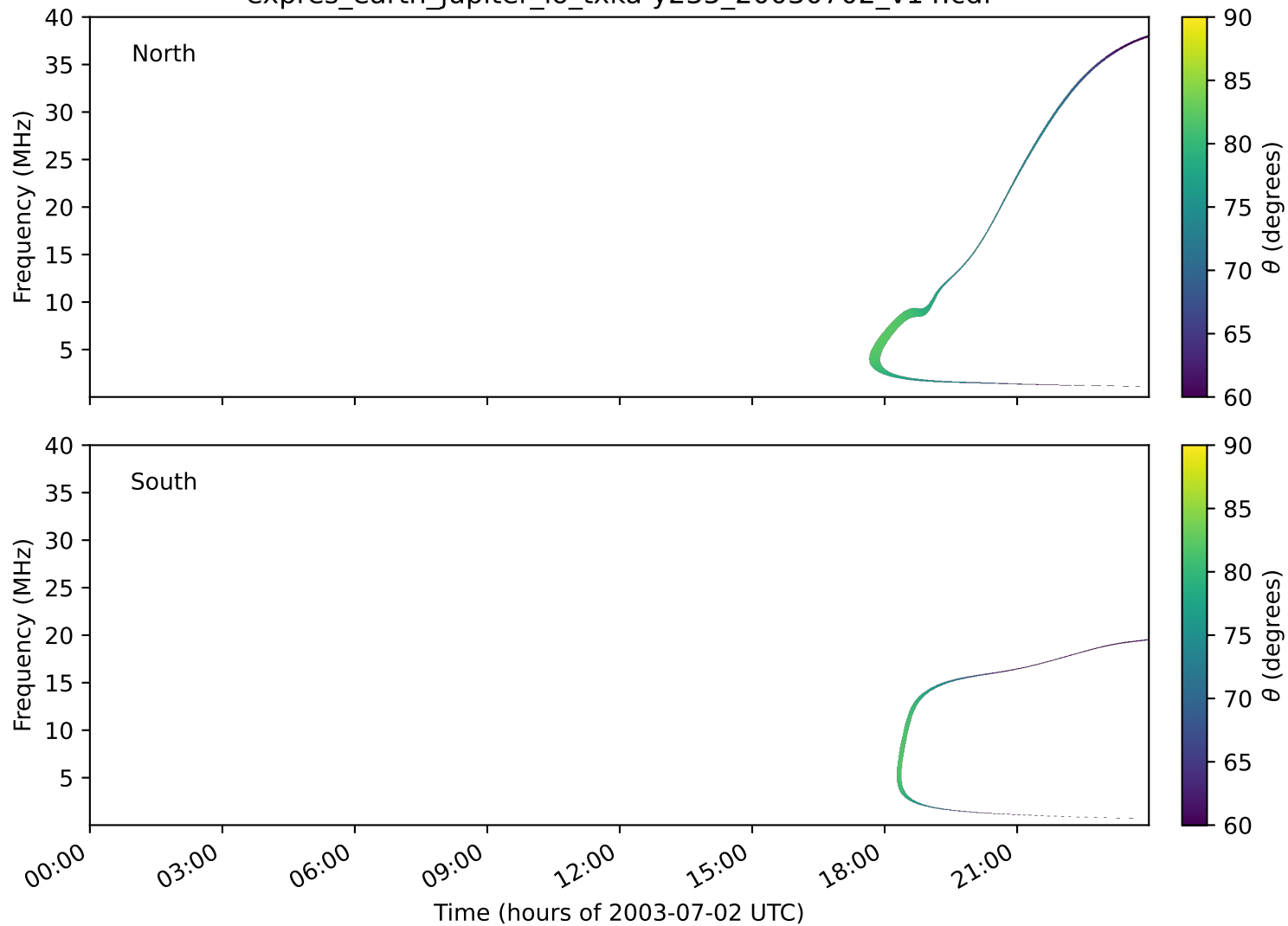
expres_earth_jupiter_io_txka-y235_20030702_v14.cdf
