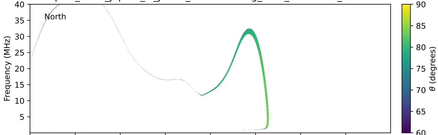
expres_earth_jupiter_io_jrm33_lossc-wid1deg_3kev_20030731_v11.cdf
