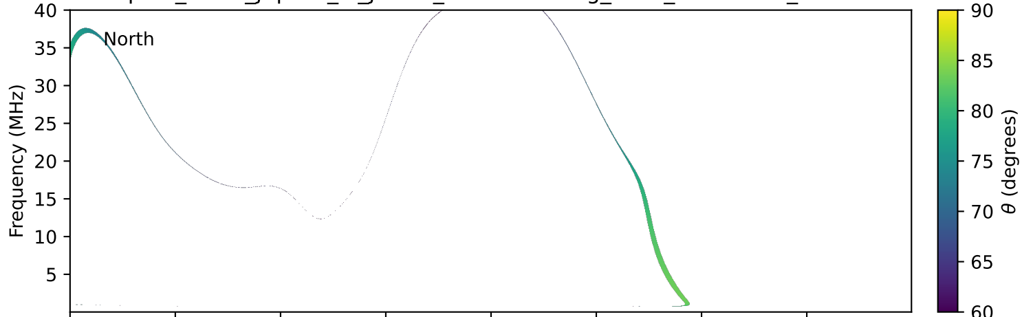
expres_earth_jupiter_io_jrm33_lossc-wid1deg_3kev_20030722_v11.cdf
