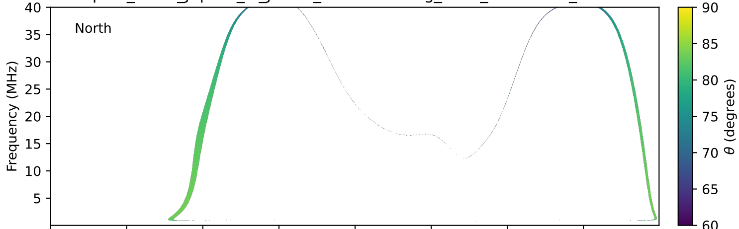
expres_earth_jupiter_io_jrm33_lossc-wid1deg_3kev_20030720_v11.cdf
