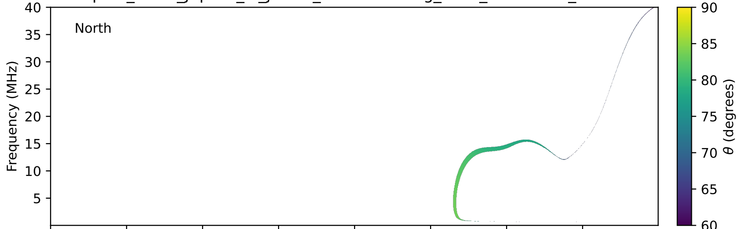
expres_earth_jupiter_io_jrm33_lossc-wid1deg_3kev_20030709_v11.cdf
