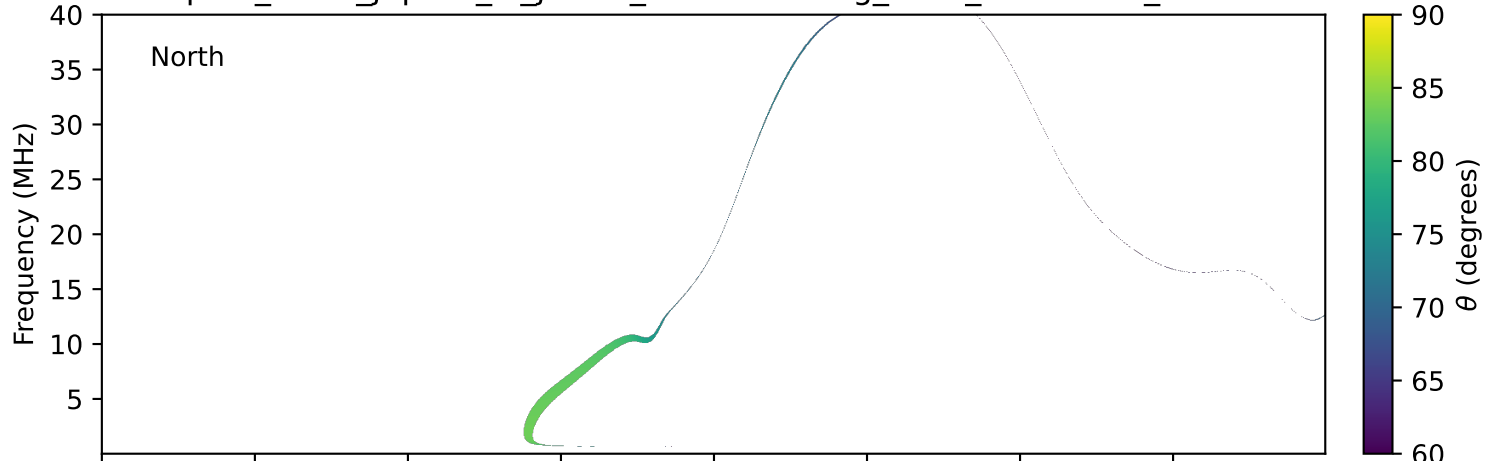
expres_earth_jupiter_io_jrm33_lossc-wid1deg_3kev_20030704_v11.cdf
