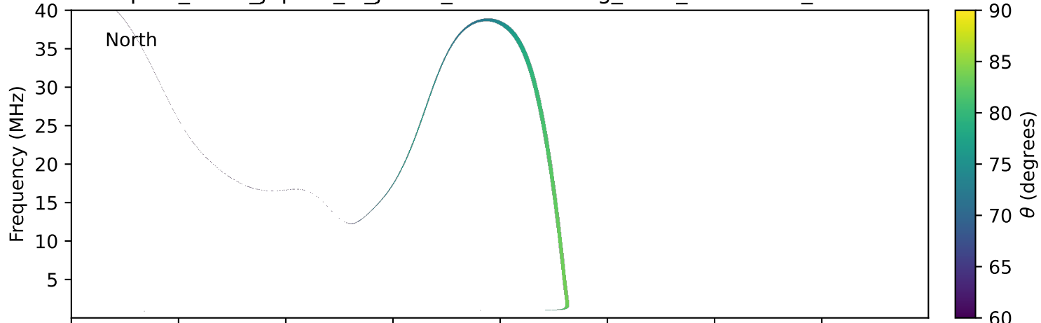
expres_earth_jupiter_io_jrm33_lossc-wid1deg_3kev_20030703_v11.cdf
